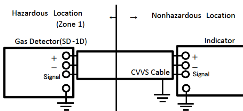
Installation Diagram
